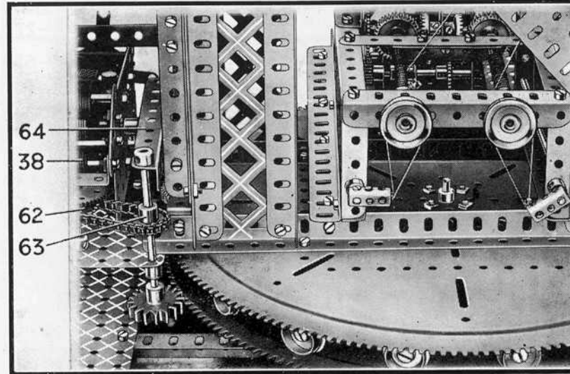
Fig 5. The fitting of the hoisting drum brakes is clearly shown in this view
