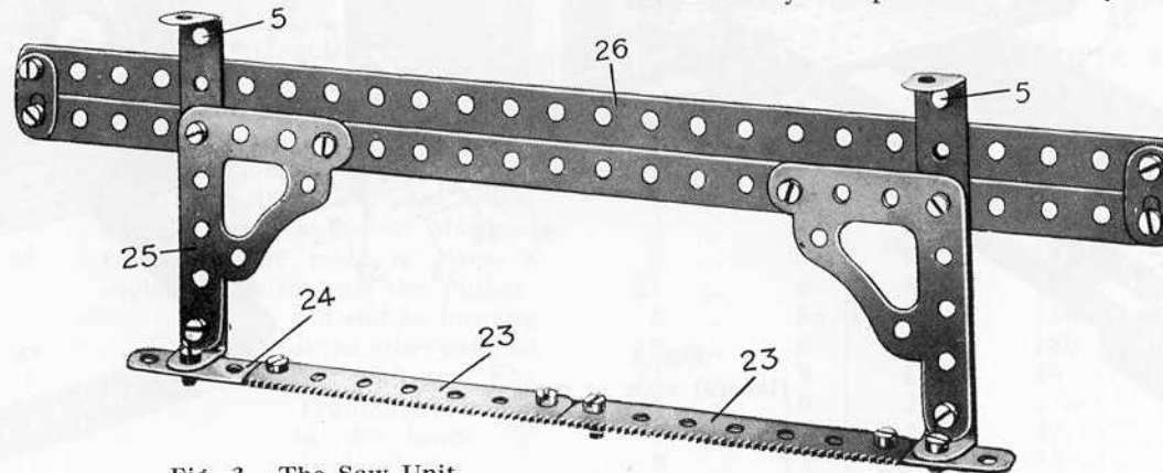
Fig. 3. The Saw Unit.
